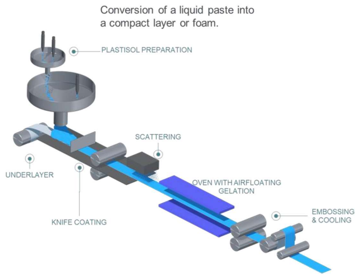
Figure 10: Coating process
